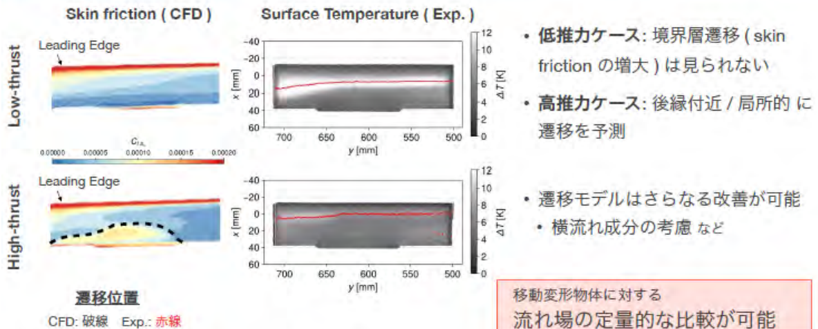
Fig: Transition location in Exp. and CFD
