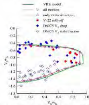
Figure 53. Calculated flight dynamics stability boundary for helicopter.
