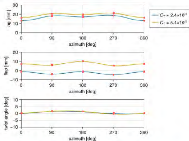
Fig: Reconstructed tip deformation
