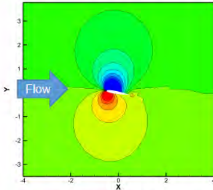
Airfoil simulation RANS, Re=3 \times 10^6 , Freestream Mach=0.2, AoA=9.6deg
