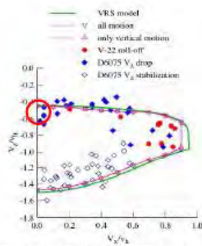
Figure 55. Calculated flight dynamics stability boundary for helicopter.
