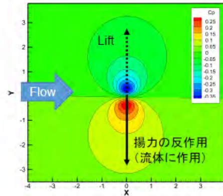
Point Source Model (The same force applied)
